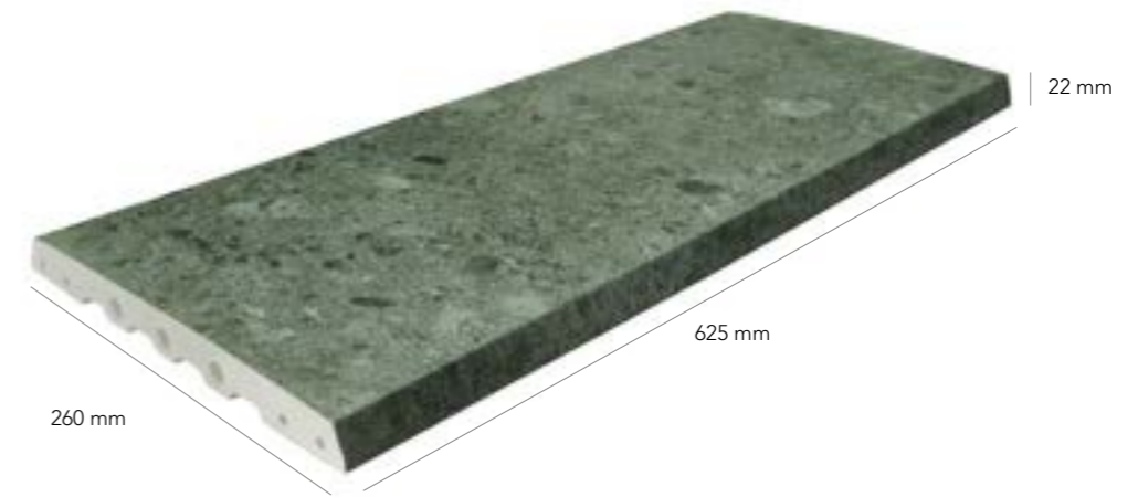
BORDE INFINITY 625 x 260 x 22
